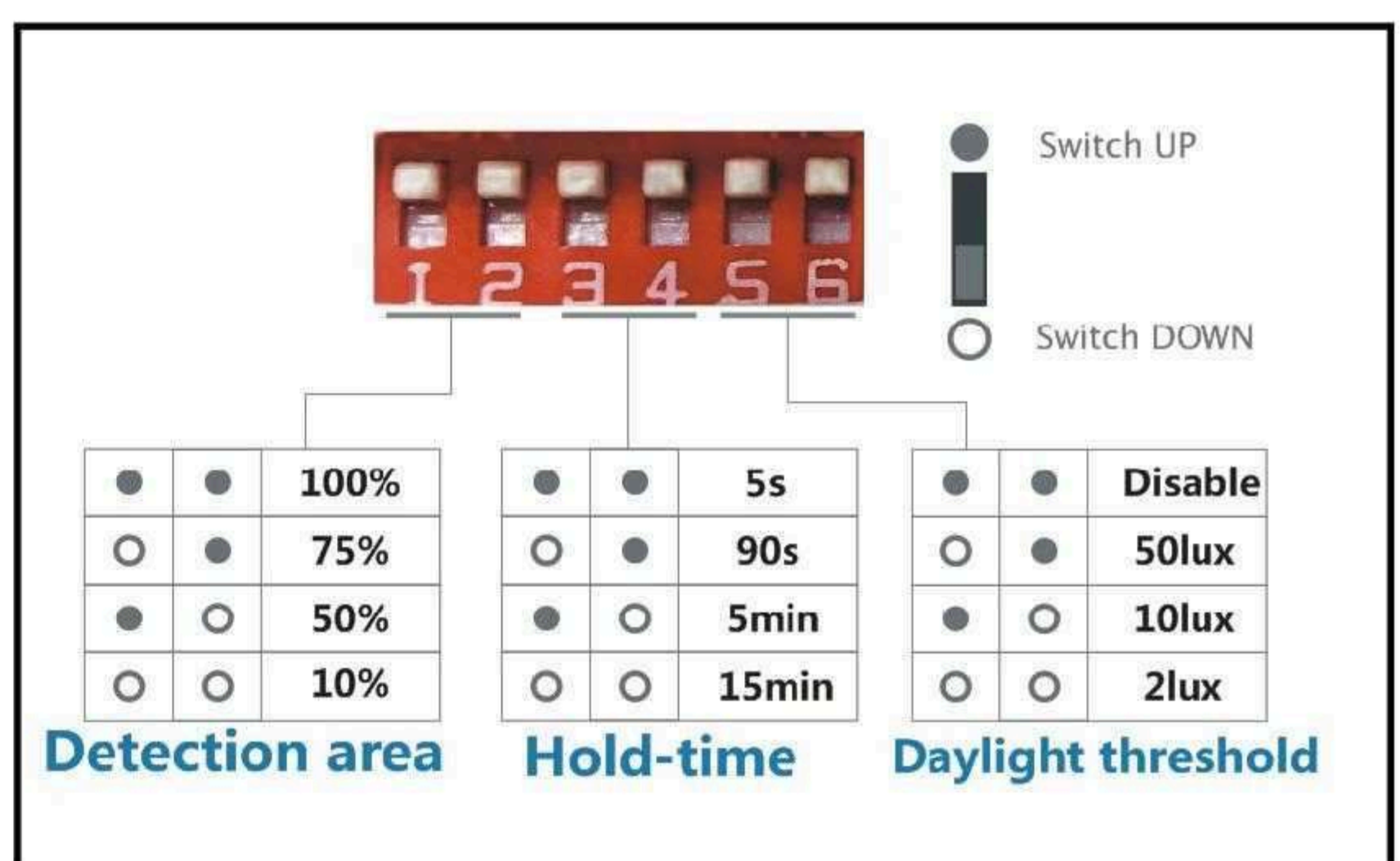
Microwave sensor
