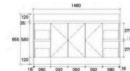
ATB-1500SA2-SD Size: 1480x450x855mm
