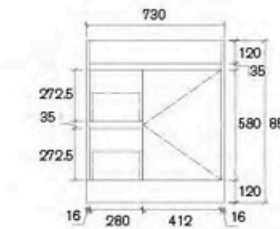
ATB-750LA1-SD Size: 730x450x855mm
