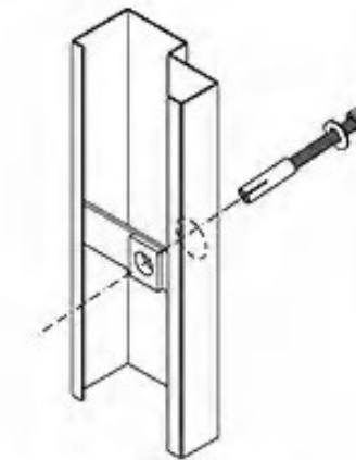
Expansion-Shell Anchor (Standard)
