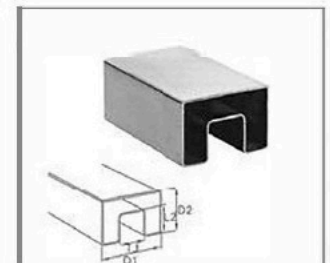
TK-1509 Rectangle Slotted Tube
