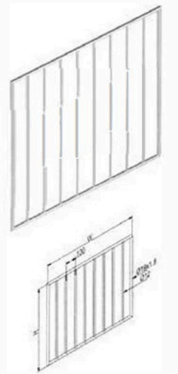
TK-F101 Material: SS304/SS316
