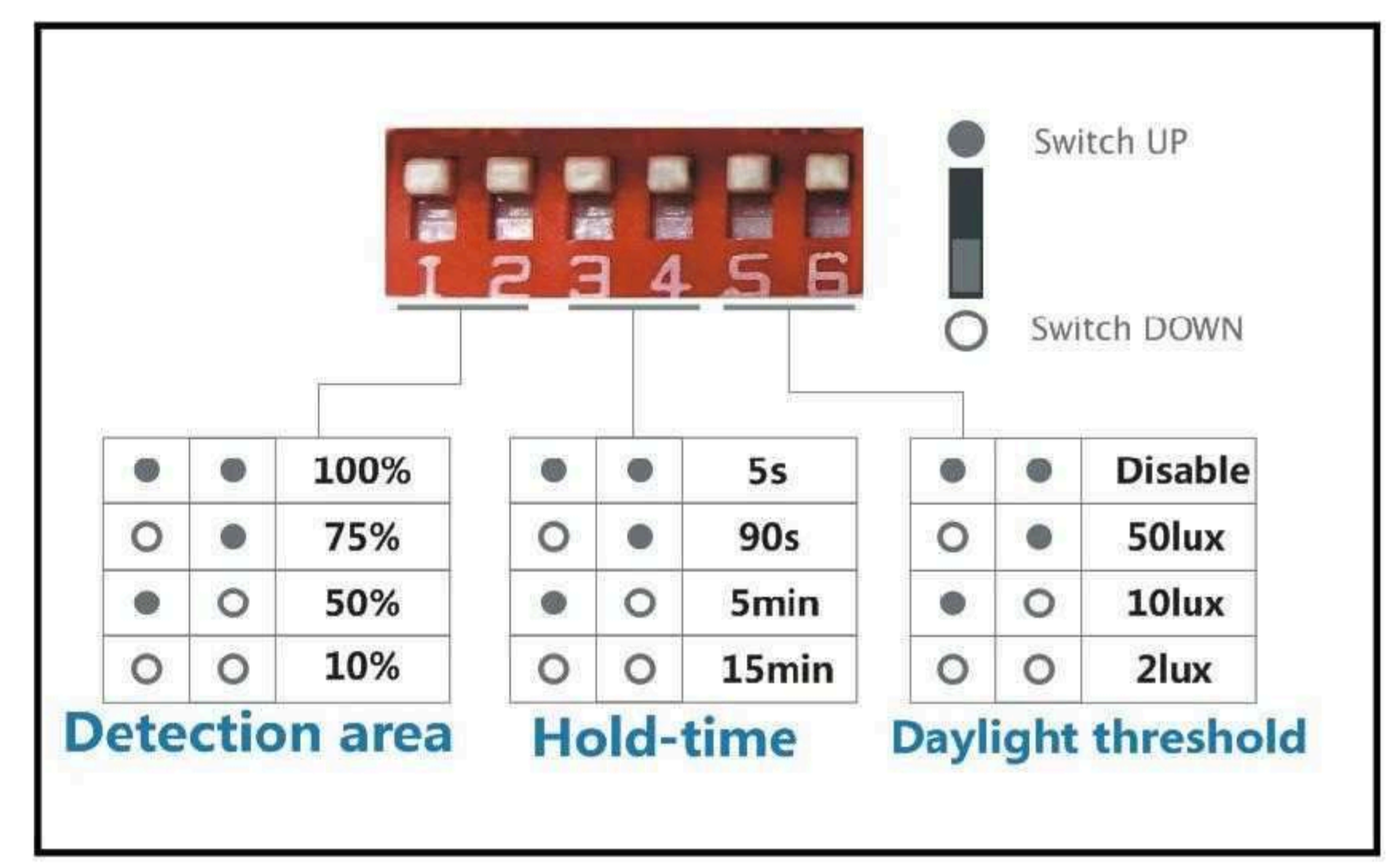
Microwave sensor
