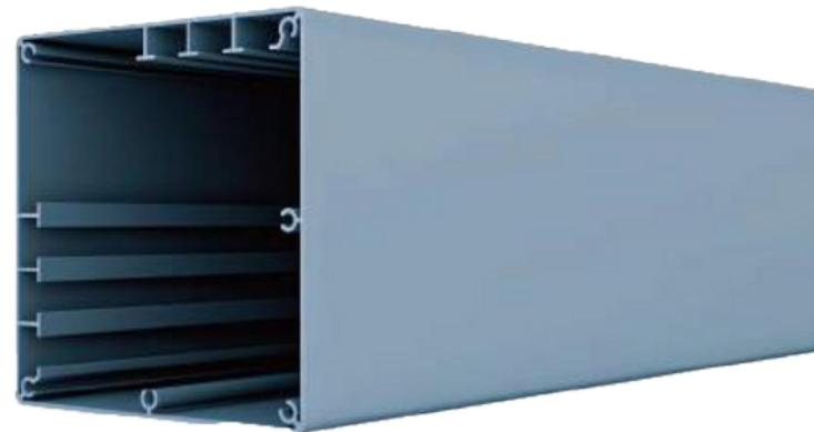
Column size: 150*150mm; Optional size: 180*180mm; Profile thickness: 2.2-3.0mm
