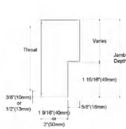
Single Rabbet
