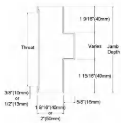
Single Rabbet
