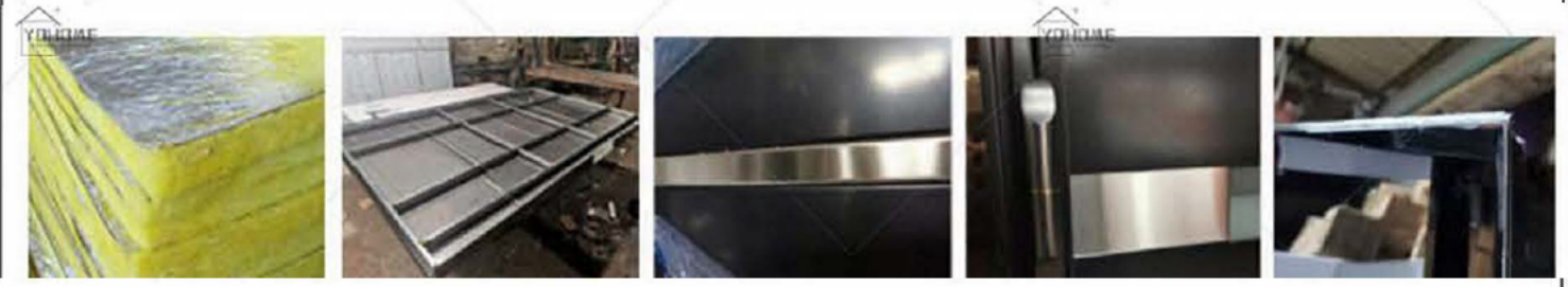
STAINLESS STEEL BOARD 10mm PLYWOOD HEAT INSULATION FOAM 10mm PLYWOOD DOOR CASE
